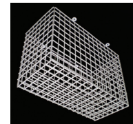
Ceiling Mount Wire Guard Part number: 2530110 Dimensions (mm) L x W x H 407 x 190 x 267
