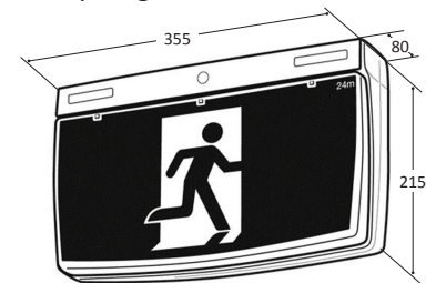
Dimensions (mm)
